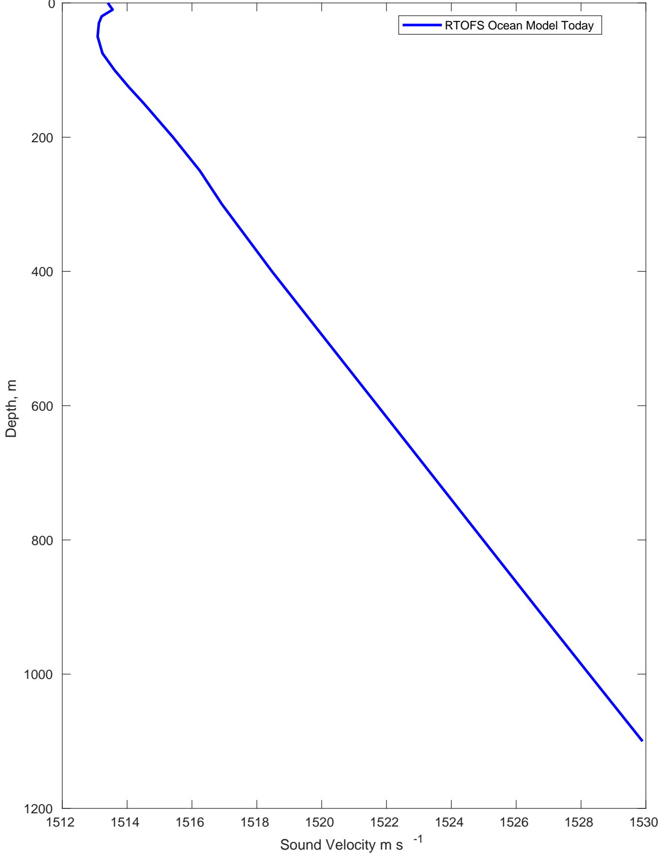
Sound Velocity Profile for Lighthouse Greece Pipeline-OSS3 on 24-Apr-2022 00:00:00
